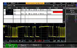
Figure 17: CAN-FD decode and trigger.
